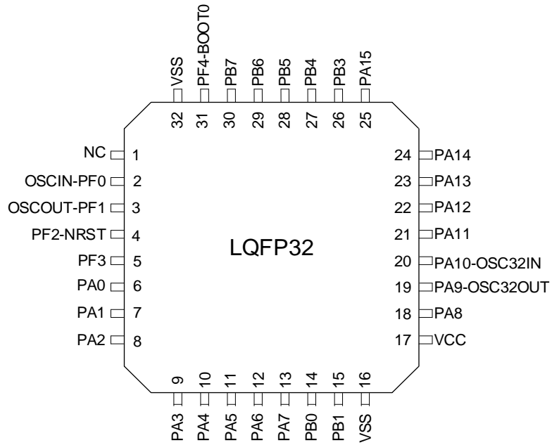
图 4-1 LQFP32 Pinout1 DM32F030K1xT
