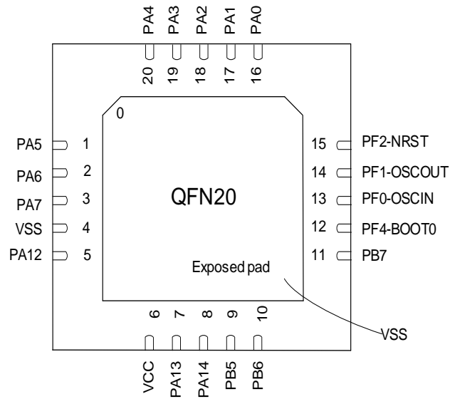
图 4-6 QFN20 Pinout2 DM32F030F2xU
