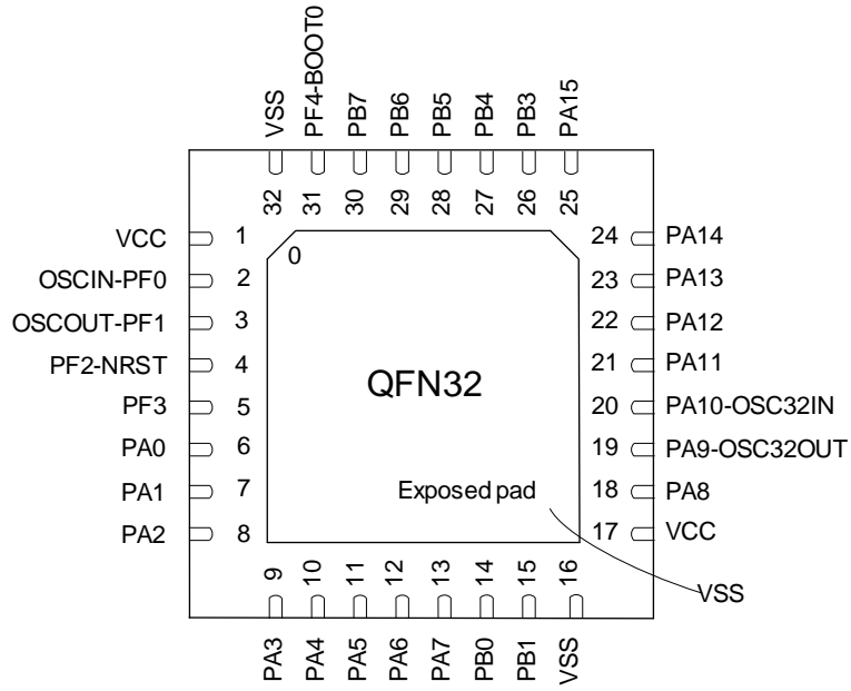
图 4-3 QFN32 Pinout1 DM32F030K1xU
