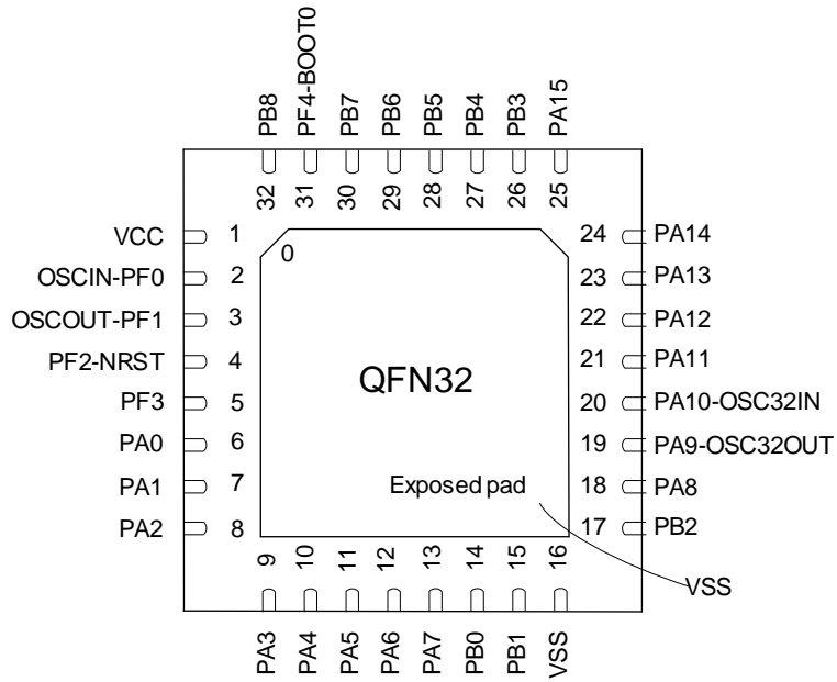
图 4-4 QFN32 Pinout2 DM32F030K2xU
