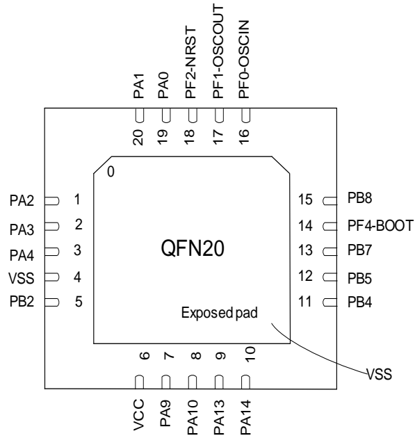
图 4-5 QFN20 Pinout1 DM32F030F1xU
