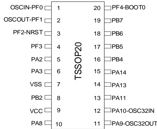
图 4-7 TSSOP20 Pinout1 DM32F030F1xP
