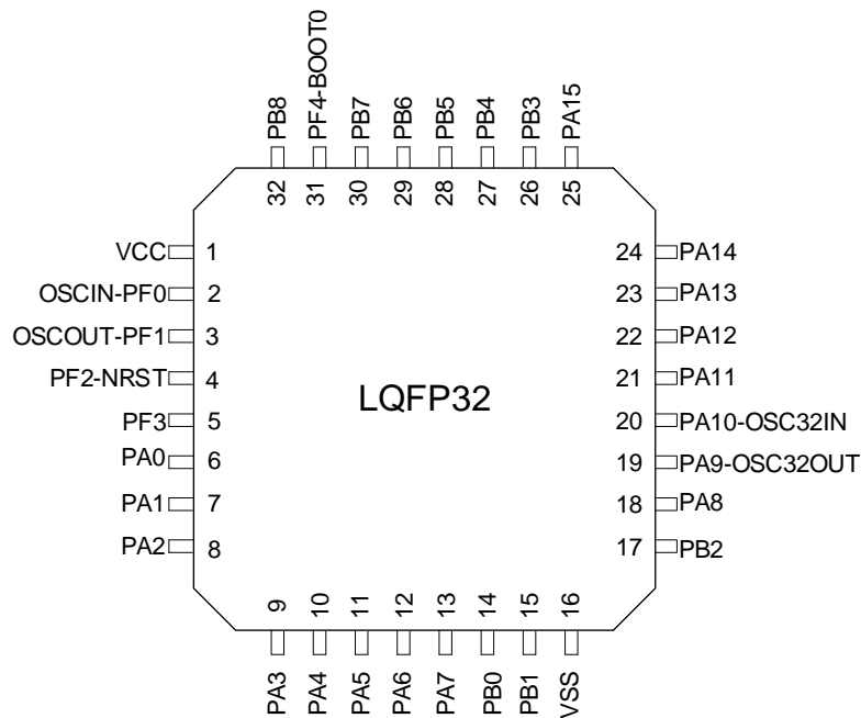
图 4-2 LQFP32 Pinout2 DM32F030K2xT
