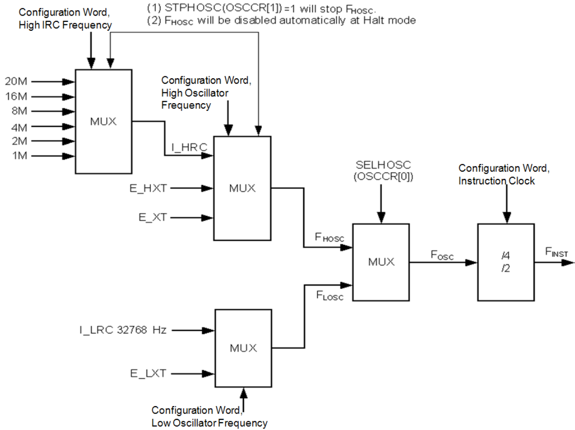
Figure 34 Oscillation Configuration of DM8P062
