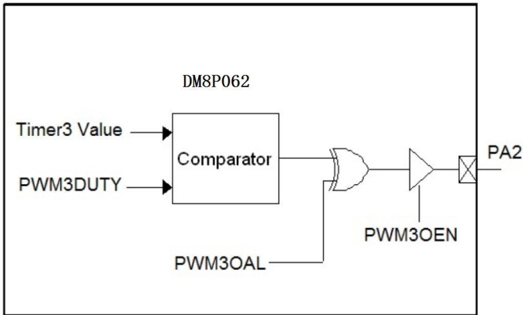
Figure 26 PWM3 Block Diagram
