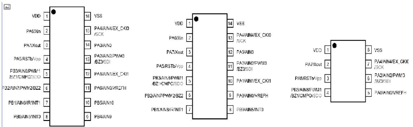
Figure 1 Package pin assignment
